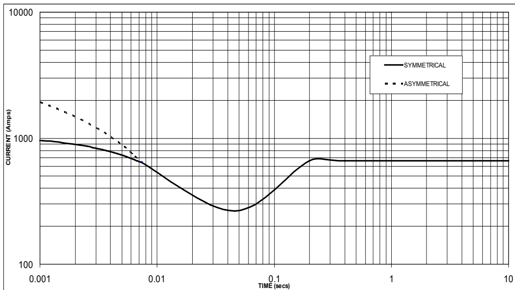
Sustained Short Circuit = 660 Amps
