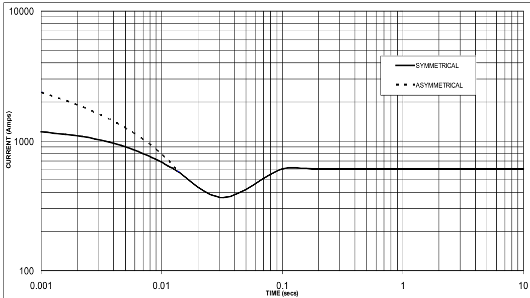
Sustained Short Circuit = 610 Amps
